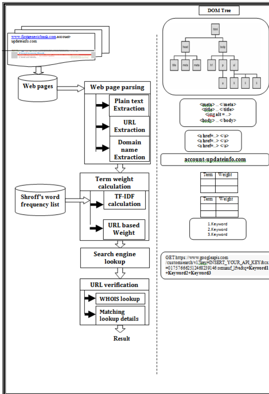
Fig.3.1: System Architecture of detecting phishing webpages.
